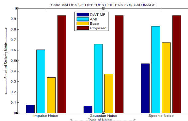
Graph. 2.SSIM values of different filters for car image
